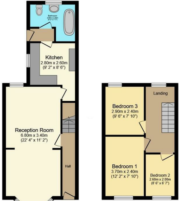
Ground Floor Floor area 44.6 sq.m. (480 sq.ft.)
