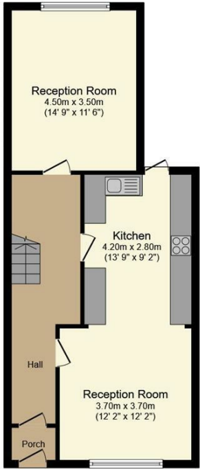
Ground Floor Floor area 56.4 sq.m. (607 sq.ft.)
